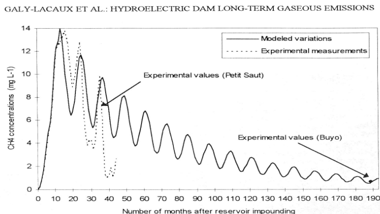
Graph 1 – Concentration Measurements and Mathematical Extrapolation of CH 4 Concentration in the Petit Saut Hydroelectric Dam Over Time
